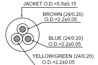
CROSS-SECTION VIEW
